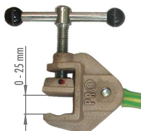
earthing clamp 823.015
